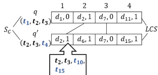
Figure 1: QDSM measure
