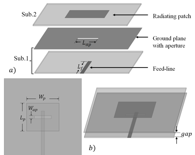
Figure 1: Single ACFP antenna structure: (a) separated components view; (b) top view and perspective view.
