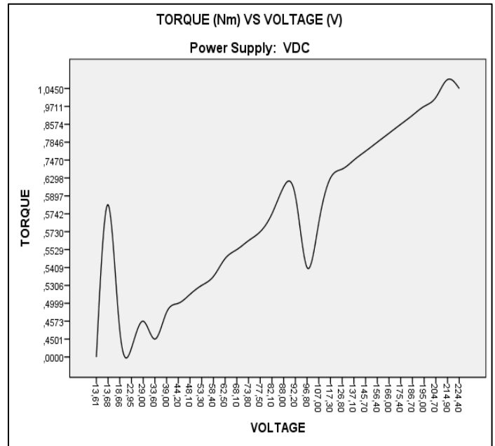
Figure 16: Analysis of Torque (N.m) and Voltage (r.m.s).
