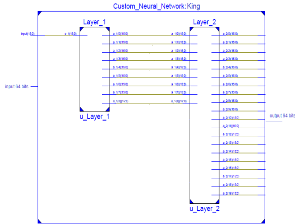
Figure 31: The RTL of king pieces used in proposed system
