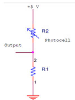
Figure 2: Constant resistance connected with LDR sensor
