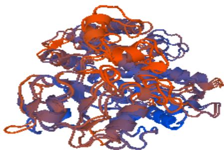
Figure 9: 1tqn.2. A
