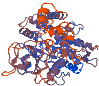
Figure 10: 4k9w.4. A
