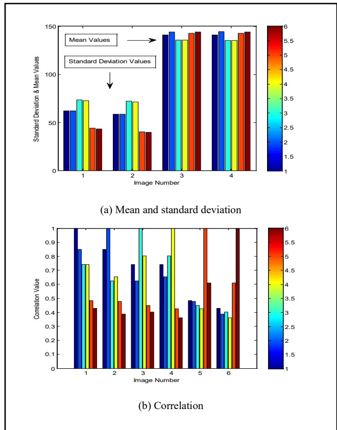
Figure 7 Statistical measures of set_2
