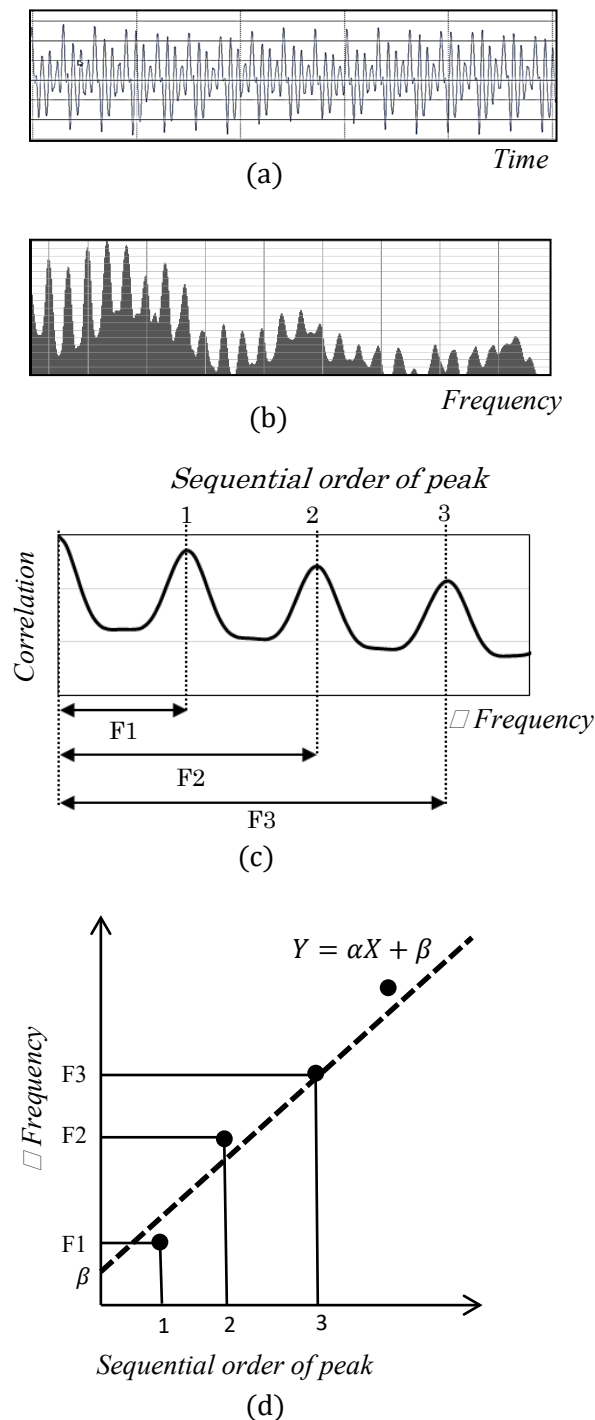
Figure 1. The pitch detection process. Details are listed in the text. (a) Voice signal, (b) frequency spectrum, (c) autocorrelation of the frequency spectrum, (d) plot of peak number and frequency shift exhibiting linear regression.
