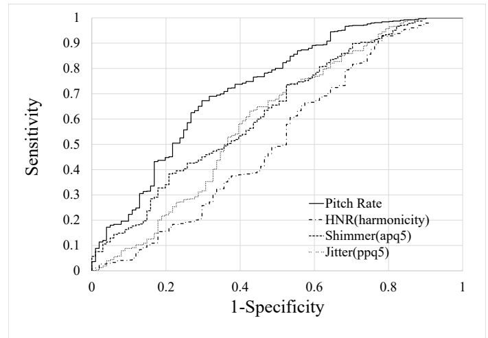
Figure 4 ROC curves used for discriminating between healthy individuals and patients using the pitch rate, jitter, shimmer, and HNR in data containing read speech of "Guten Morgen, wie geht es Ihnen?"(German).
