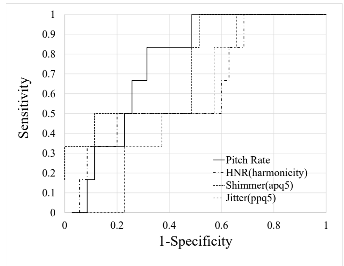
Figure 5 ROC curves used for discriminating between healthy individuals and patients using the pitch rate, jitter, shimmer, and HNR in the data containing read speech of "Kitakaze to taiyo" (Japanese).
